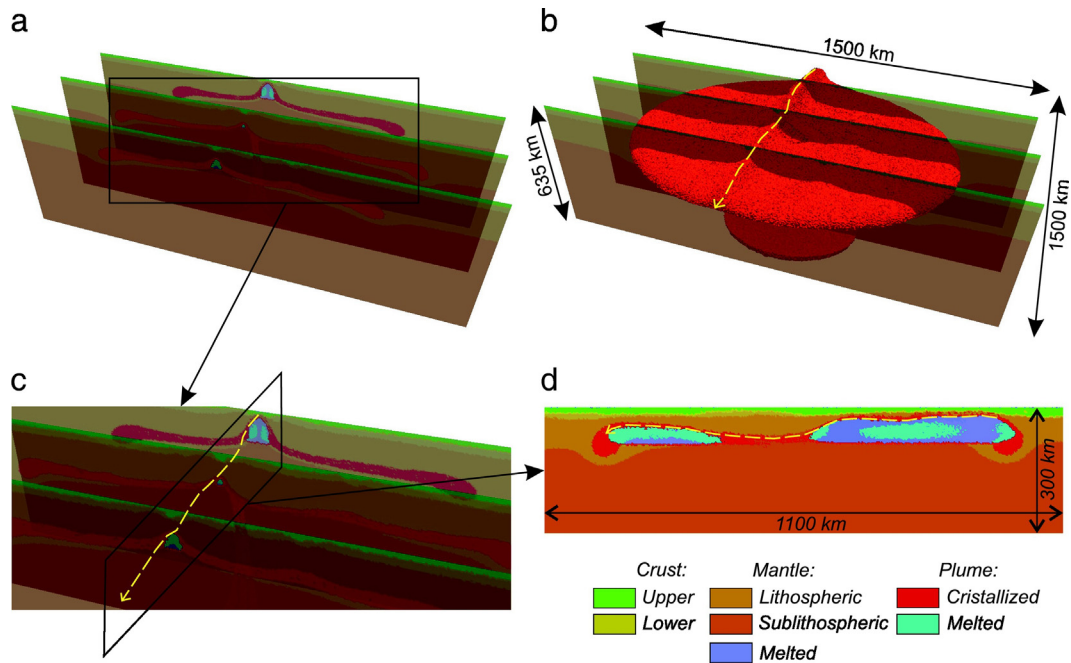
Fig. 7. Model with a mafic lower crust (Model 2). Compositional cross-sections (at 70 Myr) showing that localized plume ascent varies not only cross-strike but also along-strike. Yellow line highlights the position of the plume apex; the arrow indicates the direction of its dipping. Bulk of mantle plume is shown in red. Note that the vertical variations in the position of the plume apex reach 70–80 km that in rough accordance with conceptual model of volcanic margin segmentation based on magnetic fabric studies (Callot et al., 2001, 2002; Geoffroy, 2005; Gac and Geoffroy, 2009). See Section 4.2 for more discussion. (For interpretation of the references to color in this figure legend, the reader is referred to the web version of this article.)
