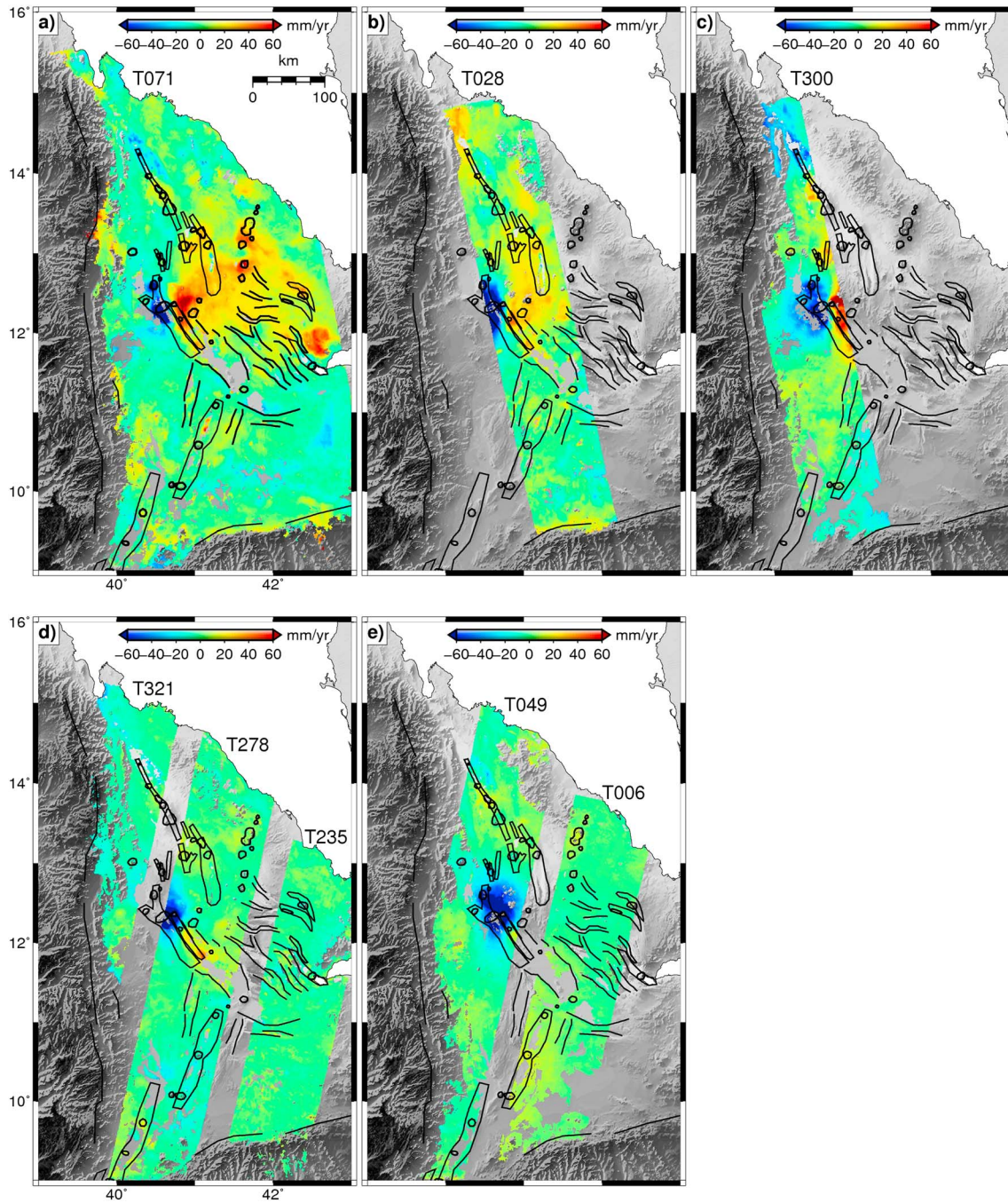
Figure 4. Average 2007–2010 LOS surface velocities for each InSAR track. The positive values indicate the range increase.
