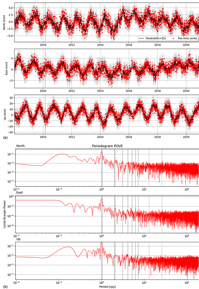
Fig. 10. Seasonal deformation at station POVE. (a) North-East-Up components time series from our processing, detrended after outlier elimination. The time series are highlighted by a Vondrak filter of cutoff frequency 25 cpy (black line). (b) Lomb-scargle periodogram of the detrended and cleaned time series over the displayed period of observation. Expected periods are represented by the vertical line (gray dashed: annual and semi-annual period; gray solid: draconitic period and harmonics; dotted line: fortnightly tidal cycle and harmonic of \sim 14 and \sim 28 days). Location of POVE is depicted in Figure 1 .
