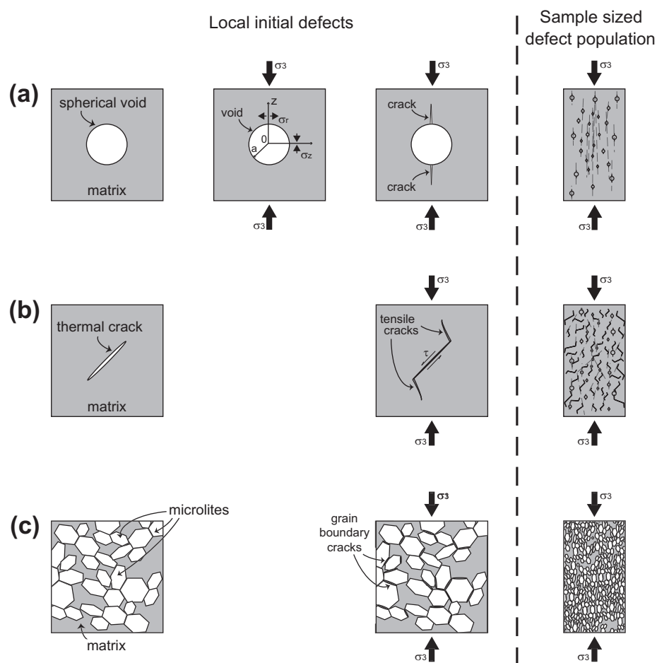
Fig. 10. Mechanisms of compressive failure in a schematic fashion: (a) case of the original glass with only spheroidal defect identified (air bubbles), (b) case of the TT glass with preexisting thermal cracks in the glass matrix, and (c) case of the Seljadur basalt with microlites in a siliceous matrix. We assume in this schematic model that \sigma_3 \ll \sigma_1 .
