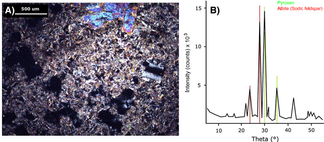
Fig. 1. Petrographical description of the Reykjanes basalt: A) thin section picture showing the microlitic texture with phenocrysts of pyroxene and the equant porosity, B) X-ray diffractogram.
