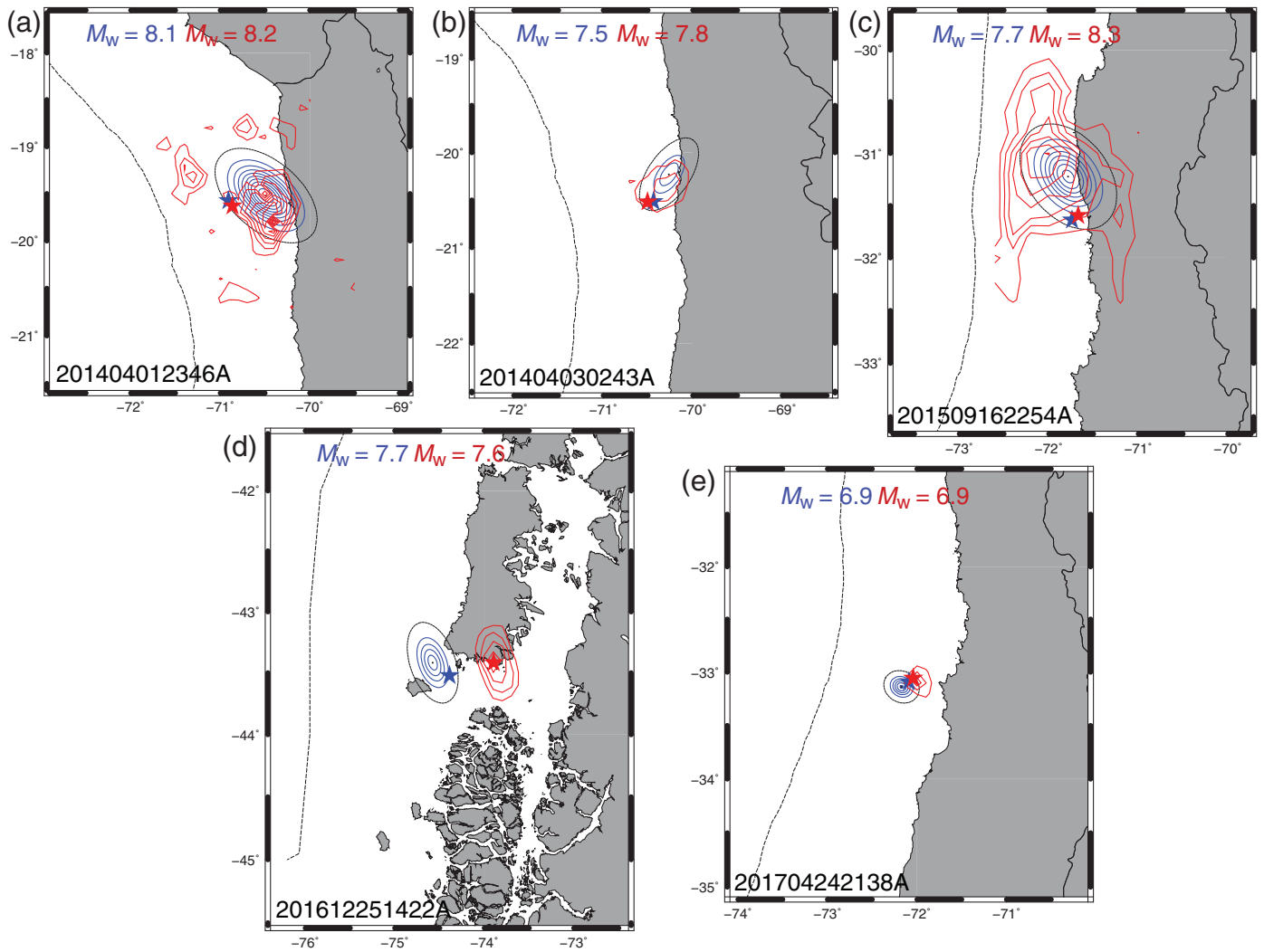
▲ Figure 4. Comparison of the slip distribution determined by this study and those of Hayes (2017) , shown with blue and red contour lines, respectively. Contour lines are plotted every 1 m in both cases, except for (e) that are plotted every 20 cm; stars represent the epicenter reported by the National Earthquake Information Center and the CSN, in red and blue, respectively. Panels presents the following events: (a) 2014 Iquique, (b) largest aftershock of the 2014 Iquique earthquake, (c) 2015 Illapel, (d) 2016 Chiloé, and (e) 2017 Valparaíso. At the top of each panel is shown the corresponding moment magnitude, in red reported by the Global CMT and in blue the one obtained in this study; at the bottom is shown its Global CMT code, for reference.
