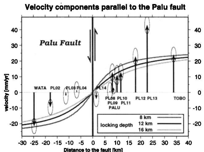
Figure 4. Transect station velocity components parallel to the fault, with the co-seismic deformation due to the Jan. 1996 earthquake removed. They are indicated in function of their distance to the fault. The dark grey line shows best model values (5.5 cm/yr total velocity, 12 km locking depth). Lighter grey lines correspond to locking depths of 8 and 16 km, marking an uncertainty of \pm 4 km.
