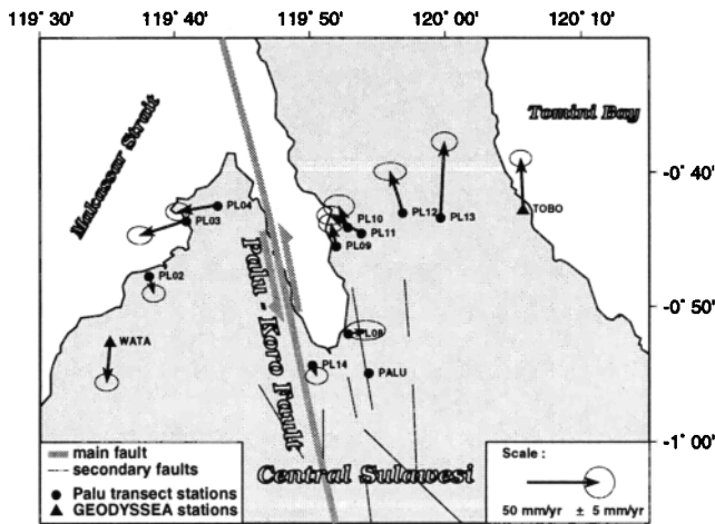
Figure 3. Velocities of the Palu transect stations, with respect to the PALU station. Error ellipses correspond to formal uncertainties of the global solution with a confidence level of 90%.
