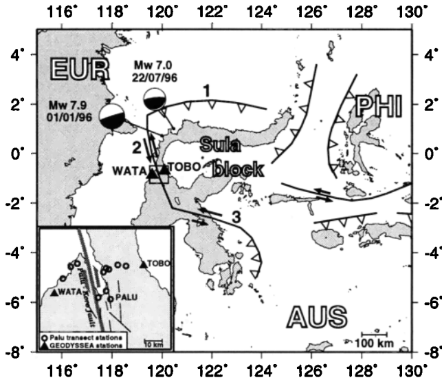
Figure 1. The area of convergence of the Eurasian, Philippine and Australian plate is characterized by the Sula block motion. Active block boundaries are the North Sulawesi trench (1), the Palu-Koro (2) and the Matano (3) faults. The Palu transect is indicated by the box, with a zoom presented in the inset. Furthermore, the two largest earthquakes (CMT) occurring during the observation period are indicated.
