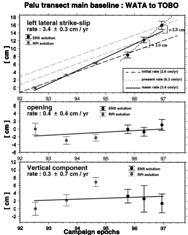
Figure 2. Time evolution of the three WATA-TOBO baseline components. Error bars indicate formal uncertainties. Straight lines represent the mean rates of motion on each component. On the strike-slip component are shown additionally an initial and a present day rate.
