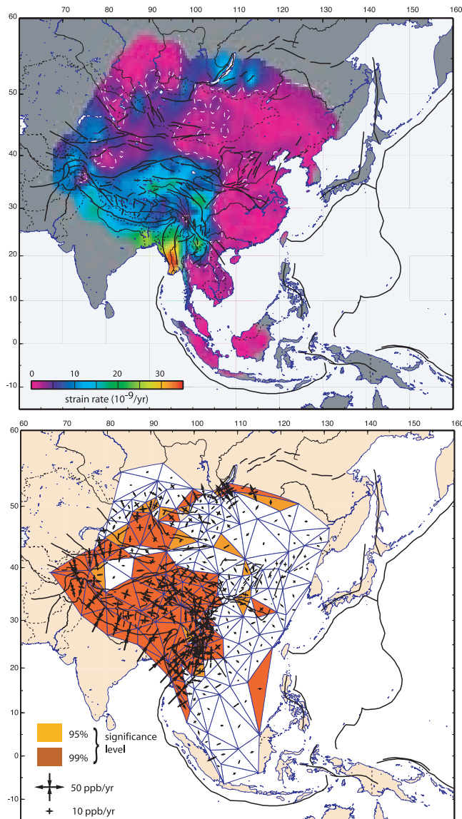
Figure 3. (top) Second invariant of the strain rate tensor calculated for a Delaunay triangulation (see Figure 2c). The white dashed line shows the 3 \times 10^{-9} \text{ yr}^{-1} contour. (bottom) Delaunay triangulation of the GPS network shown in Figure 1 with principal axis of the strain rate tensor shown at the centroid of each triangle. Convergent arrows mean contractional strain, divergent arrows mean extensional strain. Yellow and orange triangles show domains where the strain rate tensor is significant at the 95% and 99% confidence level, respectively. White triangles indicate a significance level lower than 95%.
