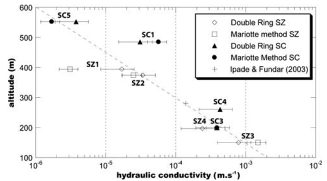
Fig. 4 Sites altitude plotted against hydraulic conductivity. Error bars are estimated to be in the order of 30% for double ring method and 50% for the Mariotte method. The value denoted K IPADE comes from Ipade and Fundar (2003). This figure highlights a relationship between altitude and hydraulic conductivities of soils: log-hydraulic conductivities are lower in high altitude than in low altitude and the trend seems to be linear
