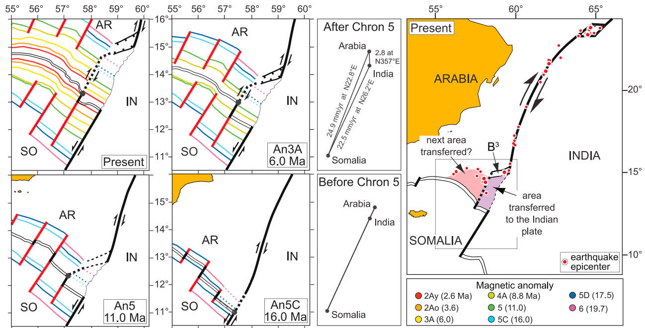
Figure 7. Four-stage evolution of the AOC triple junction at chrons 5C, 5, 3A, and present. The configuration of the junction before and after the change of geometry of the Arabia-India plate boundary is shown with the corresponding velocity space diagrams. The change in configuration was induced by a regional kinematic reorganization about 10 Ma ago (Chron 5), which initiated the formation of the Beautemps-Beaupré Basin ( B^3 ). Seismicity data suggest that, presently, a new plate boundary is developing to the west of the Beautemps-Beaupré Basin. In the near future, a larger area of the Arabian plate could be transferred to the Indian plate. AR, Arabian plate; IN, Indian plate; SO, Somalia plate.
