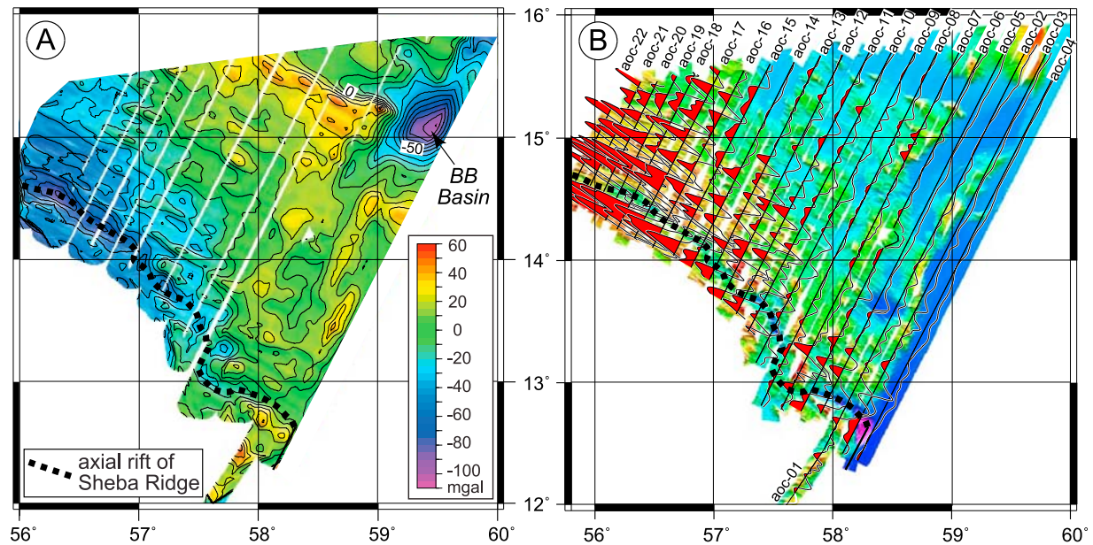
Figure 3. (a) Mantle Bouguer gravity map of the AOC triple junction computed using a mean density contrast of 1840 \text{ kg m}^{-3} between the oceanic crust and water and of 300 \text{ kg m}^{-3} between the crust and mantle. (b) Magnetic anomaly profiles plotted along ship tracks for AOC survey. High-amplitude magnetic anomalies coincide with a broad negative mantle Bouguer anomaly. Both gravity and magnetic data were acquired along the ship tracks with an original data spacing of 30 m along track and \sim 17 \text{ km} ( \sim 9 nautical miles) between tracks.
