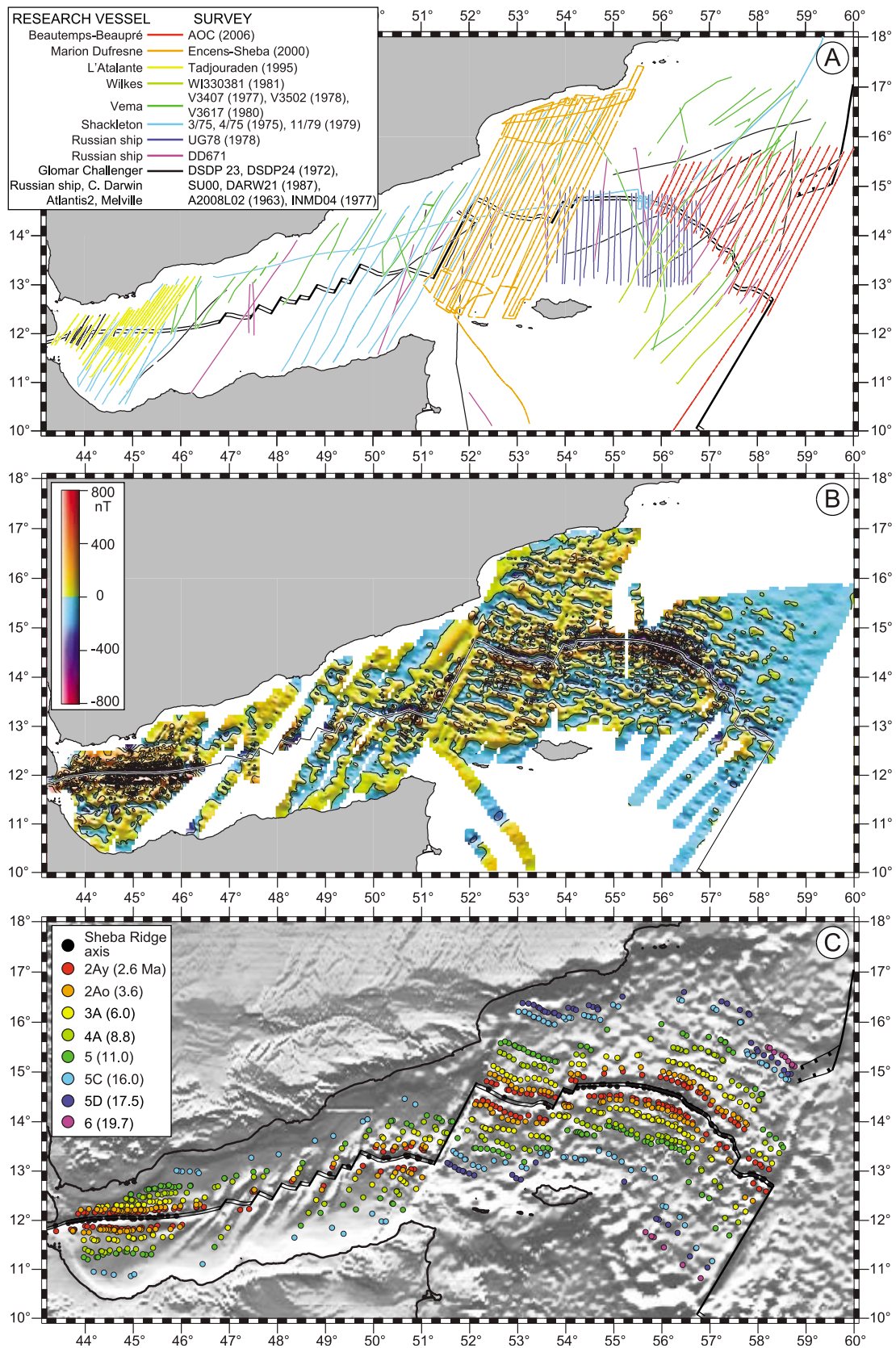
Figure 8. (a) Location of ship tracks for magnetic profiles used in this study. (b) Contoured magnetic anomaly amplitude map of the Gulf of Aden. Contour interval, 200 nT. (c) Magnetic anomaly picks including the central anomaly and anomalies 2Ay, 2Ao, 3A, 4A, 5, 5C, 5D, and 6. Anomaly 5C (16.0 Ma) can be traced in most of the Gulf of Aden.
