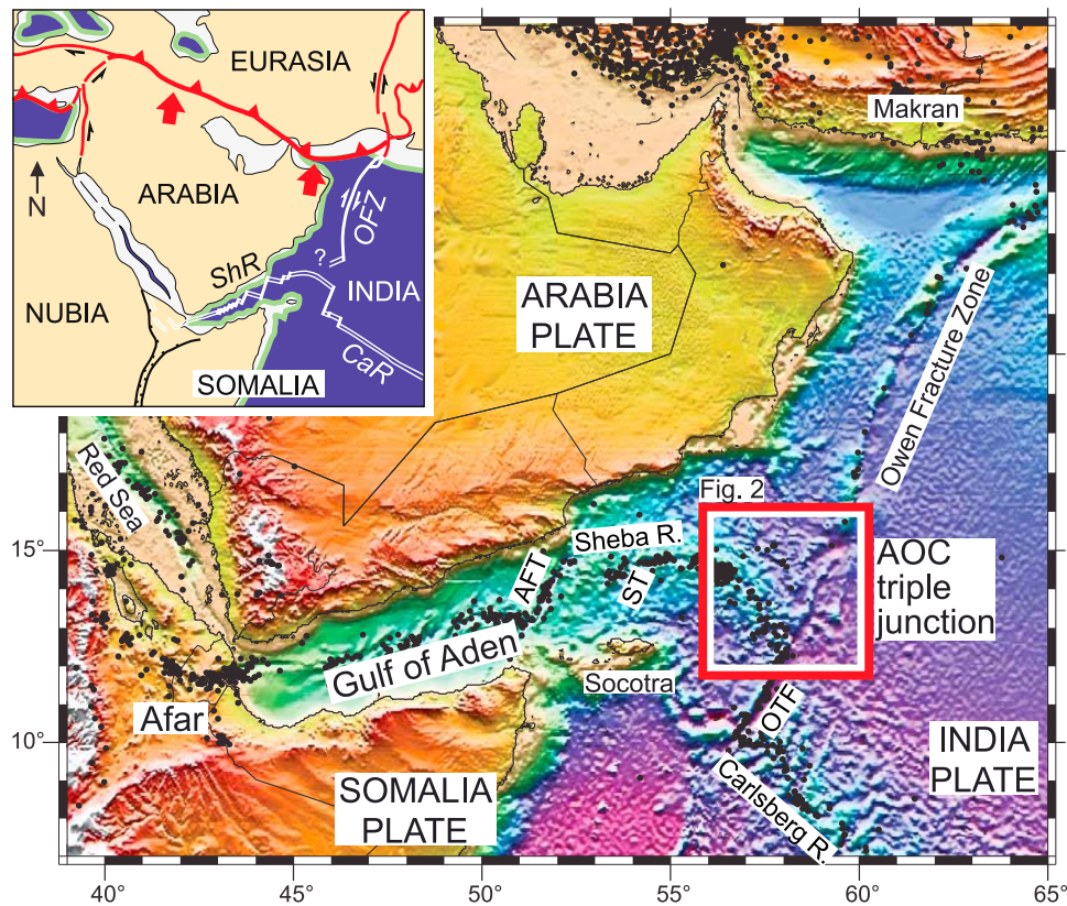
Figure 1. Geodynamic framework of the Gulf of Aden between the Afar hot spot and the Aden–Owen–Carlsberg (AOC) triple junction. Satellite altimetry data from Sandwell and Smith [1997] and shallow seismicity since 1973 from USGS/NEIC database (focal depth < 50 km; magnitude > 2). Inset shows the plate tectonics setting. AFT, Alula–Fartak transform fault; CaR, Carlsberg Ridge; OFZ, Owen fracture zone; OTF, Owen transform fault; R, ridge; ShR, Sheba Ridge; ST, Socotra transform fault.
