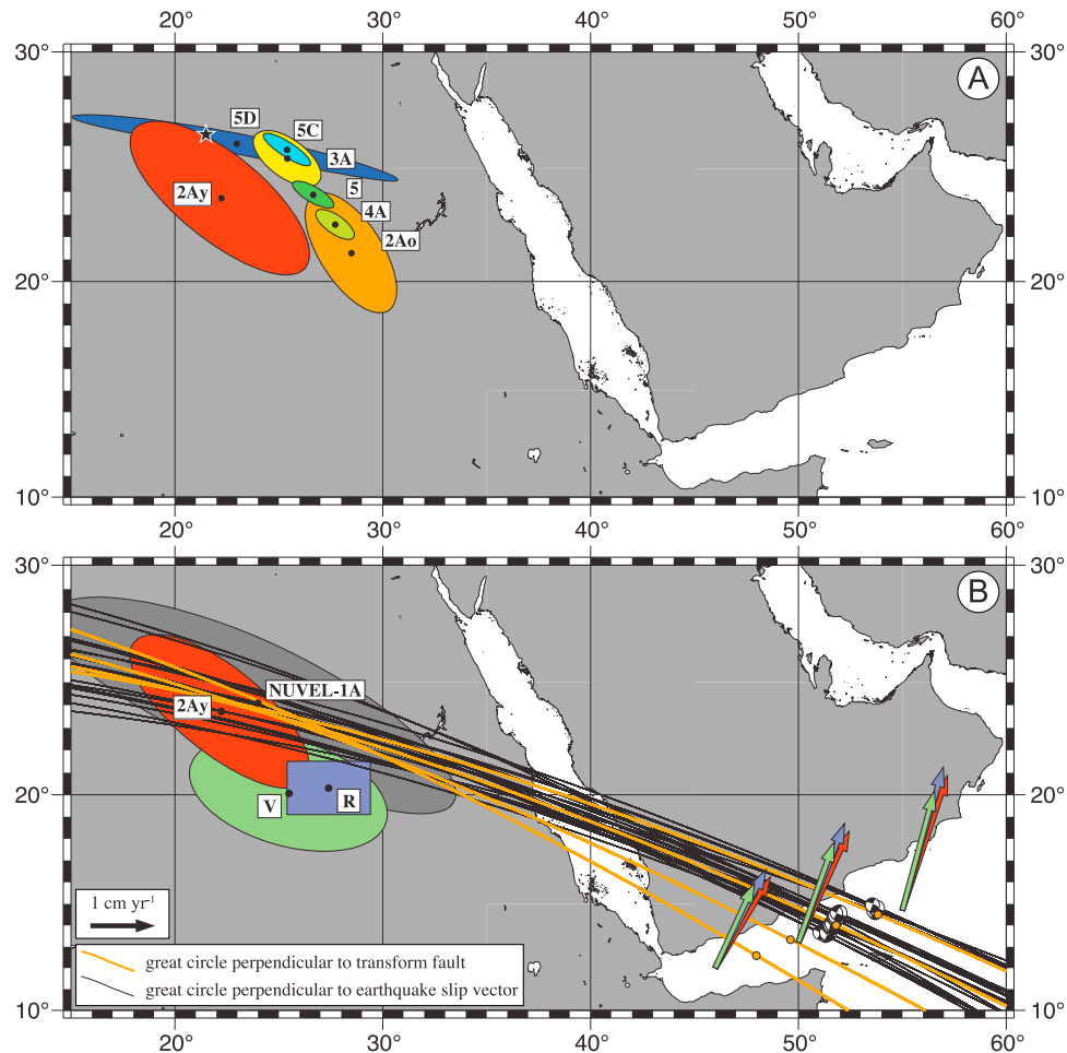
Figure 9. (a) Kinematics of the Gulf of Aden calculated from seafloor spreading magnetic anomalies: Arabia-Somalia finite rotation poles with their 2-sigma error ellipse (Table 1) and finite rotation pole to close the Gulf of Aden (star) [McKenzie et al. , 1970]. Since Chron 5D, the rotation poles migrated southeastward toward the Gulf of Aden. (b) Arabia-Somalia instantaneous kinematics: comparison between “geodetic” and “geologic” kinematics with an independent data set (azimuths of transform faults and earthquake slip vectors). Rotation poles calculated from GPS data (R [Reilinger et al. , 2006] and V [Vigny et al. , 2006]) and from magnetic data (NUVEL-1A and Chron 2Ay) are plotted with their 2-sigma error ellipses, together with rates predicted along the Sheba Ridge (arrows). Great circles perpendicular to transform faults and earthquake slip vectors (Table 3) should intersect near the rotation pole [Morgan, 1968].
