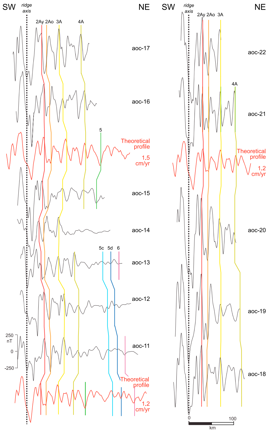
Figure 4. AOC survey magnetic anomaly profiles projected along N27°E and aligned along the Sheba Ridge axis. Location of profiles is shown in Figure 3b. Theoretical anomaly profiles were generated using the magnetic inversion time scale of Cande and Kent [1995; see also Sloan and Patriat , 1992] with a magnetized layer of 400 m which follows the seafloor topography and a contamination factor of 0.7. The “y” or “o” suffixes of magnetic anomalies indicate the young or old edge of the chron, respectively.
