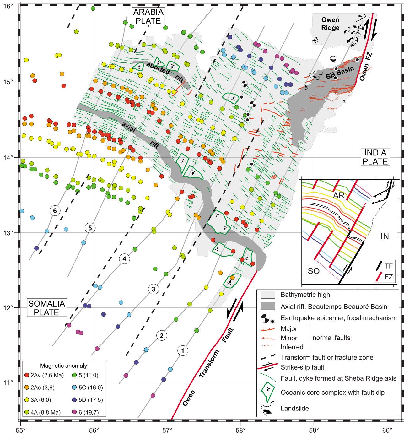
Figure 6. Magnetic anomaly picks plotted on the structural map of the AOC triple junction. Two segments separated by a major transform fault are recognized. Along the western segment, magnetic anomalies are identified from anomaly 2Ay to 6 on both flanks of the ridge. Along the eastern segment, magnetic anomalies are identified from anomaly 2Ay to 6 on the southern flank and from anomaly 2Ay to 5 on the northern one. In the central part of the western segment, the anomaly 5, which is an important marker usually recognized with certainty, is not clearly identified (profiles aoc-11 to aoc-14 in Figure 4). To the west of the Beautemps-Beaupré Basin, NW-SE-trending faults and dykes formed at the Sheba Ridge are crosscut by E-W faults, suggesting that the extensional deformation has propagated westward. Inset shows the isochron map with the present-day geometry of plate boundaries. AR, Arabian plate; FZ, fracture zone; IN, Indian plate; SO, Somalia plate; TF, transform fault.
