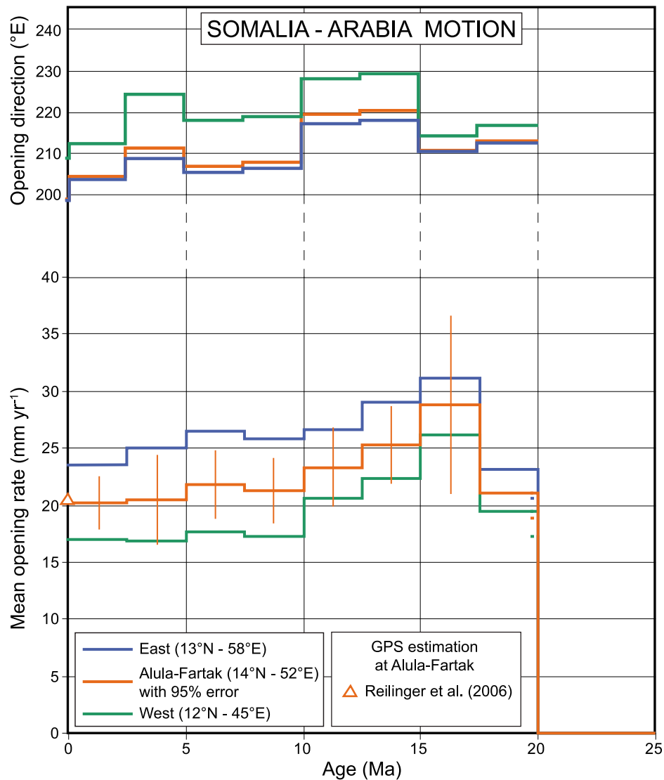
Figure 10. Variation of the opening rate and direction (with respect to Arabia) through time for three different portions of the accreting boundary: western ( 12^{\circ}\text{N} , 45^{\circ}\text{E} ), central ( 14^{\circ}\text{N} , 52^{\circ}\text{E} ; Alula-Fartak transform fault), and eastern ( 13^{\circ}\text{N} , 58^{\circ}\text{E} ; AOC triple junction area) Gulf of Aden. Stage poles every 2.5 Myr are derived from the original stage poles (Table 2). The slow and gradual decrease of the spreading rate during the last 10 Myr is not in line with a 15–20% decrease during the last 3 Myr, as suggested by GPS data [Vigny et al. , 2006].
