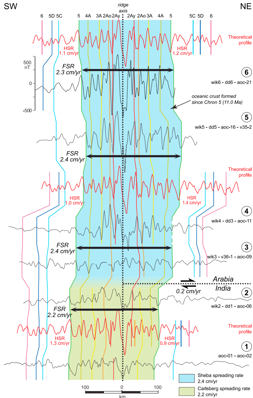
Figure 5. Six full magnetic anomaly profiles across the eastern Gulf of Aden reconstituted from V3502 and V3617 (R/V Vema), WI330381 (R/V Wilkes), DD671 (Russian ship), and AOC (R/V Beautemps-Beaupré) surveys. The profiles are projected along N27°E and aligned along the Sheba Ridge axis. Location of profiles is shown in Figure 6. Since Chron 5 (11.0 Ma), oceanic floor was generated at a full spreading rate of 2.4 cm yr -1 along the western segment (in blue referred to as “Sheba rate”) and of 2.2 cm yr -1 along the eastern segment (in green referred to as “Carlsberg rate”). The relative motion of 2 mm yr -1 is accommodated by right-lateral slip along the transform zone between the two segments. Same legend as Figure 4. HFS, half-spreading rate for theoretical profiles; FSR, full spreading rate.
