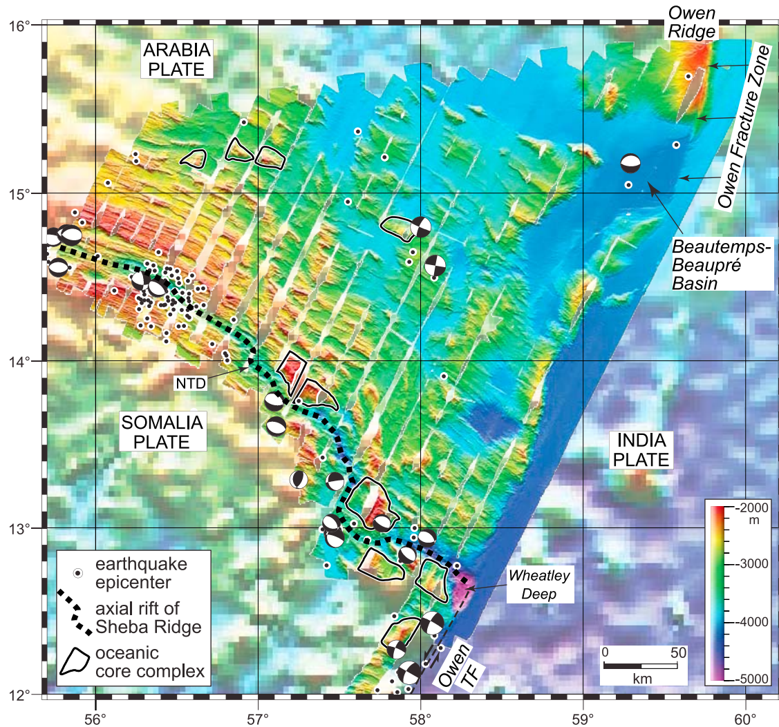
Figure 2. Multibeam bathymetric data of the AOC triple junction (location in Figure 1) superimposed on the world bathymetric map of Sandwell and Smith [1997] with shallow seismicity and earthquake focal mechanisms (Global CMT catalog). The map shows the northern flank of the Sheba Ridge and its axial rift, and the southern termination of the Owen fracture zone in the Beautemps-Beaupré Basin. NTD, nontransform discontinuity; TF, transform fault.
