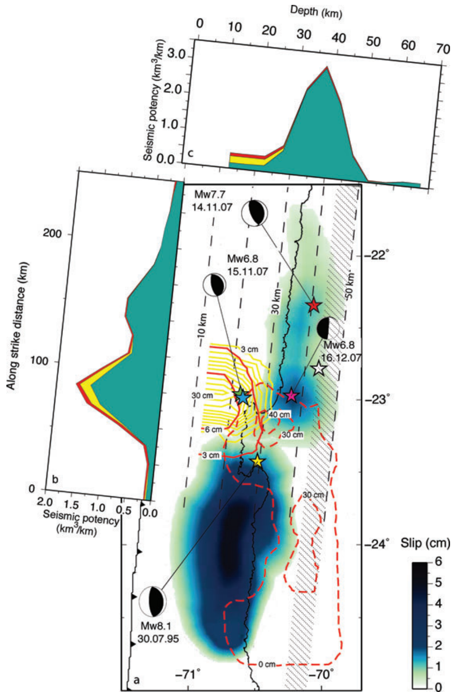
Figure 7. Comparison between the coseismic and post-seismic slip from the 1995 Mw 8.1 Antofagasta and 2007 Mw 7.7 Tocopilla earthquakes. (a) Magnitude of coseismic slip on the fault interface is represented by the colour palette for the 1995 and the 2007 earthquakes. Yellow and red solid contours represent slip distribution for the two large aftershocks and the first post-seismic period studied (cGPS-post1) following the Tocopilla earthquake, respectively. Contour interval is 3 cm in both cases. Red dashed contours (10-cm interval) represent 5-yr aseismic post-seismic deformation that followed the 1995 Antofagasta earthquake. Epicentre for both subevents of the main shock (red and white stars) and three large aftershocks (blue, green and pink star) and their focal mechanism from Peryat et al. (2010) are indicated. Epicentre (yellow star) and focal mechanism for the 1995 Antofagasta earthquake (from Monfret et al. 1995 and the Harvard CMT solution, respectively) are also indicated. (b) and (c) Seismic potency (product of ruptured area and slip) per kilometre along strike and along dip, for the coseismic (green area), November 15 aftershock (yellow area) and post-seismic (red area) models associated with the 2007 Tocopilla earthquake. The total geodetic moment for this model can be determined by summing the potencies and multiplying the sum by the value of the shear modulus of the Earth's crust (assuming an averaged shear modulus of 33 GPa moment values are those indicated in Table 2). Depths on the fault interface are shown as black dotted lines labelled every 20 km. The depth interval where the continental Moho intersects the subduction interface is shown as a striped area (Patzwahl et al. 1999).
