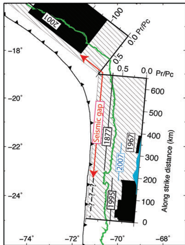
Figure 8. Seismic potency deficit along strike in the North Chile–South Peru subduction zone after the Tocopilla earthquake. Striped area represents interseismic potency cumulated (Pc) since 1877 in the North Chile gap and 1968 in the South Peru gap for a 100 per cent locking of the thrust interface between the Nazca and South American plates during the interseismic period and 6.4 \text{ cm yr}^{-1} of convergence rate (Angermann et al. , 1999). Blue area represents the seismic potency released (Pr) during the 2007 Tocopilla main shock, its two M_w \geq 6 aftershocks on 2007 November 15 and the two post-seismic periods studied (cGPS-post1 and cGPS-post2). Black areas represent the seismic potency released during other M_w \geq 7 earthquakes occurred in the region (see Fig. 1). Note that several M_w \geq 7 in the region of Antofagasta ( M_w 7.5 1987, M_w 7.0 1988, M_w 7.2 1988 and M_w 7.1 1998) are included in the Pr estimation, although they are not labelled. In the case of the 1995 Antofagasta, 2001 Arequipa and 2007 Tocopilla earthquakes, the seismic potency released during the post-seismic period is also included (20 per cent of the coseismic moment for the M_w 8.1 Antofagasta earthquake, Chlieh et al. 2004; Pritchard & Simons 2006; 40 per cent of the coseismic moment for the M_w 8.4 Arequipa earthquake, Ruegg et al. 2001; Melbourne et al. 2002; Pritchard 2003; 5 per cent of the coseismic moment for the 2007 Tocopilla earthquake, this work). Question marks indicate that the potency cumulated before the 1995 earthquake is uncertain in this region. Coastline (green line) and trench (barbed line) have been superposed as reference.
